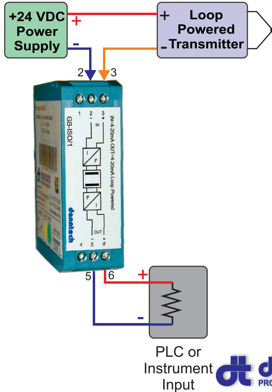
Loop-Powered Transmitter Input
