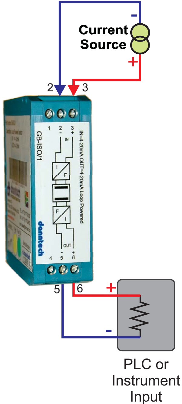
Self-Powered Transmitter Input
